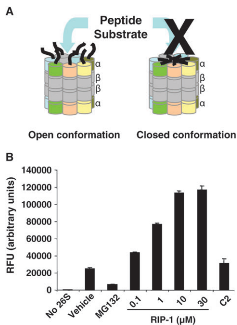
Fig. 2 RIP-1 stimulates 26S proteasome-mediated peptidolysis. (A) Hydrolysis of an unfolded peptide substrate by the 26S proteasome is inhibited by a 'flap' structure comprised of the N-terminal tails of the 20S CP \alpha sub-units that occlude the opening into the catalytic interior of the complex (right). The ATPases of the 19S CP (not shown here) must hold these peptides in an 'open' conformation in order for the substrate to diffuse into the barrel. (B) Effect of RIP-1, MG132 and a control peptoid, C2, on this activity. Vehicle denotes the solvent in which the peptoids were dissolved.
